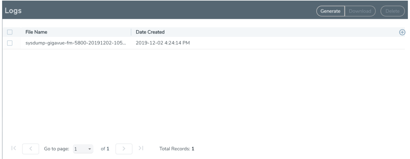
Figure 23 Logs Page
